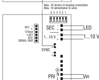
1...10 V diagram - Collegamento 1...10 V
